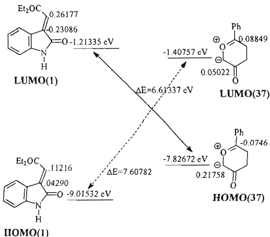
Figure 7. The correlation diagram for the reaction of 1 with carbonyl ylide 37
