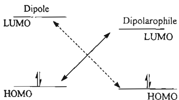
Type 1 (HOMO Controlled)
