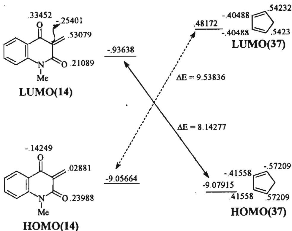
Figure 3. The correlation diagram for the reaction of 14 with cyclopentadiene
