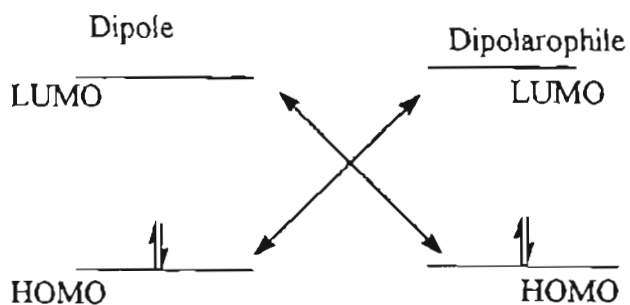
Type 2 (HOMO-LUMO Controlled)
