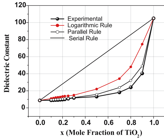
FIGURE 3 Variation of \epsilon_r of \text{MgAl}_2\text{O}_4 with a \text{TiO}_2 addition
