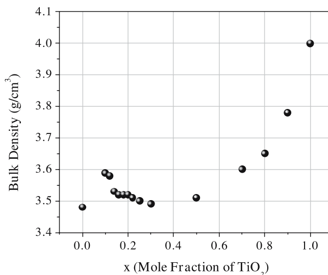
FIGURE 1 Variation of bulk density of MgAl 2 O 4 with a TiO 2 addition
